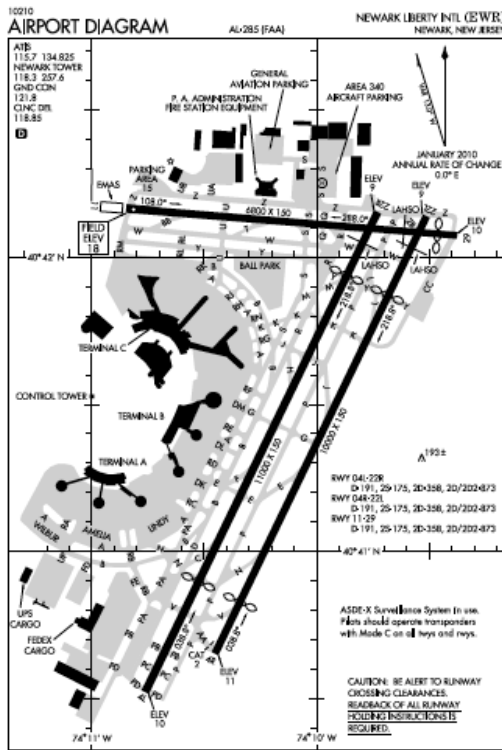
Figure 2. EWR Runway Layout [14]
