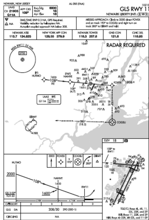
Figure 3. GLS Runway 11 Approach Procedure [14]
