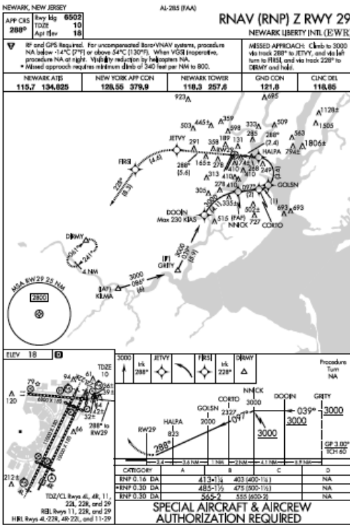
Figure 5. RNAV(RNP) Runway 29 Approach Procedure [14]
