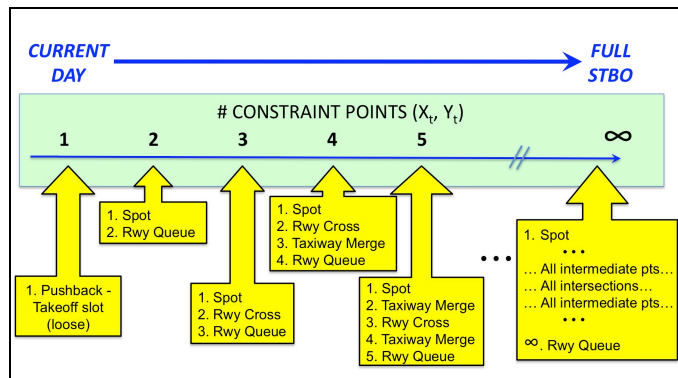
Figure 1. Variants of the STBO concept related to the STBO taxi clearance. STBO taxi clearances may have one or two (left) or an infinite number (right) of time “constraint points” – locations along the taxi clearance route that have an associated required time of arrival (RTA).
