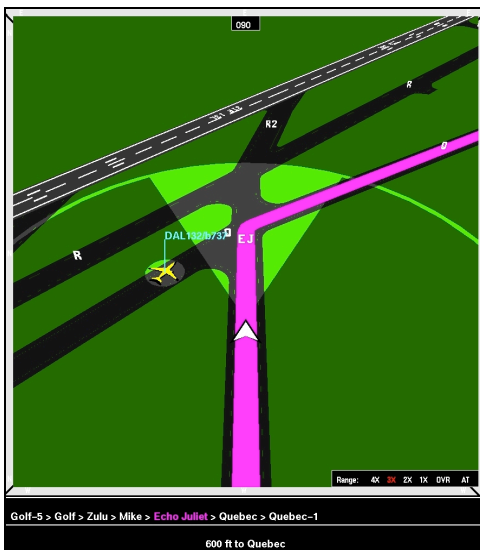
Figure 8. Taxi Navigation Display (TND).
