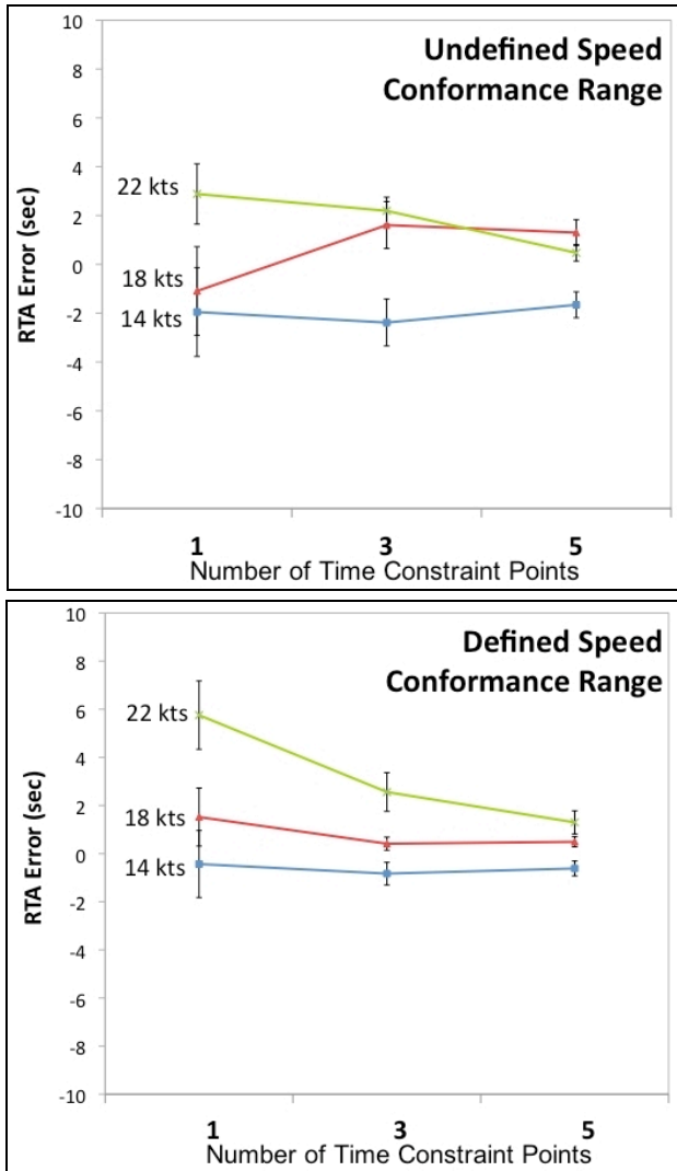
Figure 10. Mean required time of arrival (RTA) error as a function of commanded speed and number of time constraint points for the Undefined and Defined speed conformance conditions. Error bars = +/- 1 standard error.
