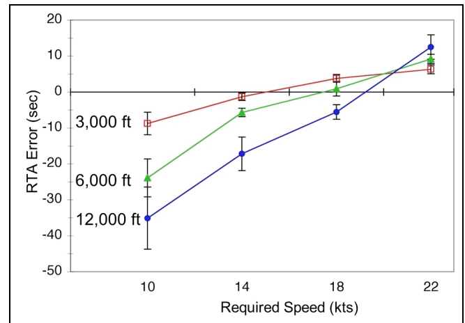
Figure 4. Mean required time of arrival (RTA) error by distance and required speed, averaged across display format. Error bars = +/- 1 standard error.
