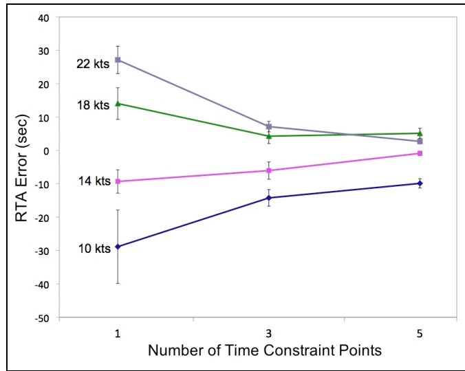
Figure 9. Mean required time of arrival (RTA) error as a function of commanded speed and number of time constraint points. Error bars = +/- 1 standard error.
