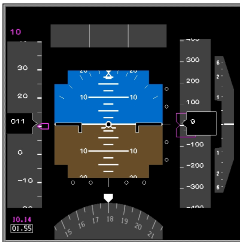
Figure 12. Prototype NextGen PFD. Speed tape (left) shows Commanded Speed = 10kts; Current Speed = 11kts. Elapsed taxi time = 1:55 min/sec; Total required taxi time = 10:14 min/sec.)
