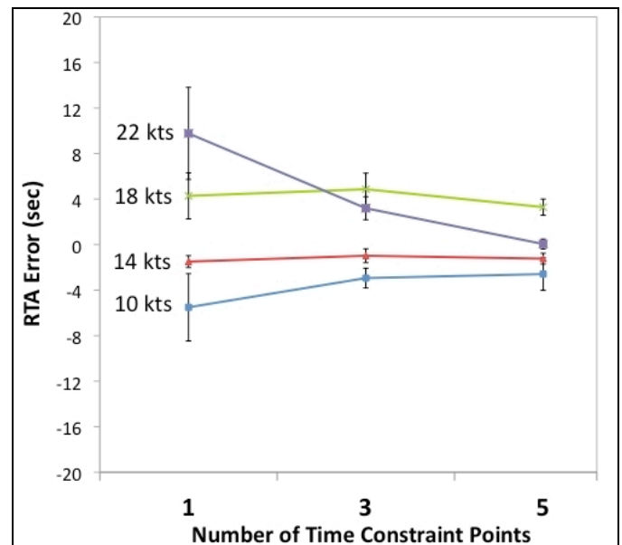
Figure 13. Mean required time of arrival (RTA) error as a function of commanded speed and number of time constraint points. Error bars = +/- 1 standard error.
