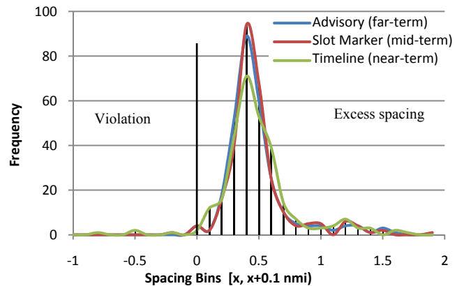
Figure 5. Inter-arrival spacing between consecutive aircraft measured at the runway threshold, by tool condition.
