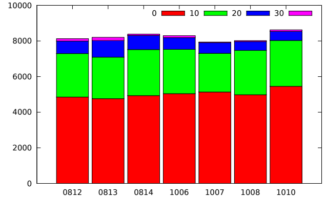
Fig. 4. Distribution of discrepancies from RFL after allocation.
