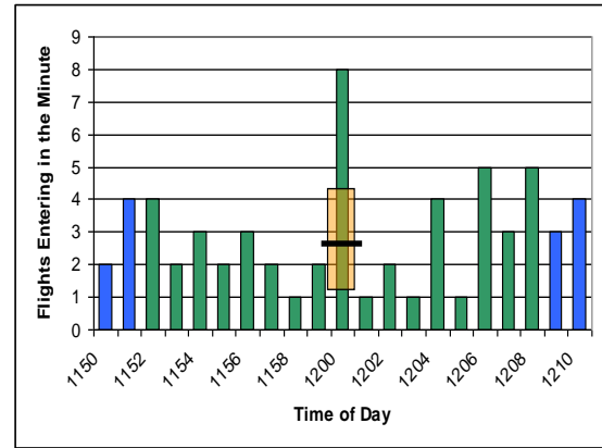
Figure 3-2 Sector Entry Counts
