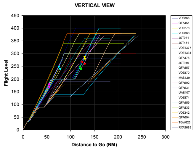
Figure 8. YMML arrivals 09-10 UTC – CTA scenario.
