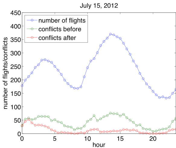
Figure 10. Flights and conflicts during July 15, 2012
