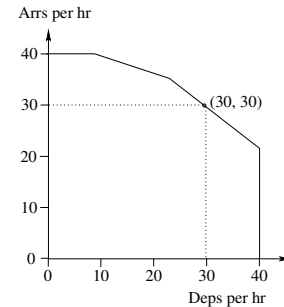
Figure 2: An airport runway capacity envelope with four segments.
