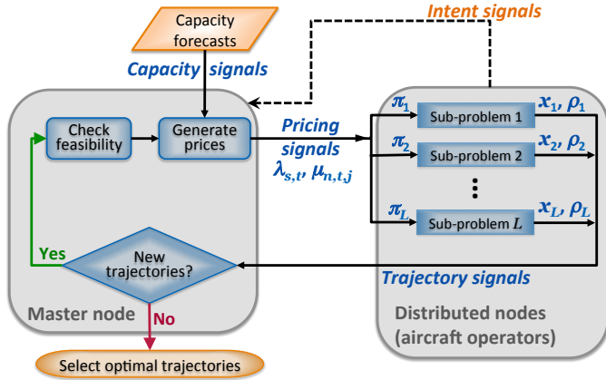
Figure 4: Schematic of the distributed solution process for very large-scale ATFM [11].
