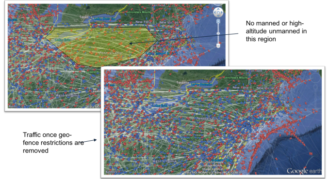
Figure 8: Example of geofence implementation using DRIFT, showing traffic unmanned (red) and manned (blue) traffic, with and without geofencing.
