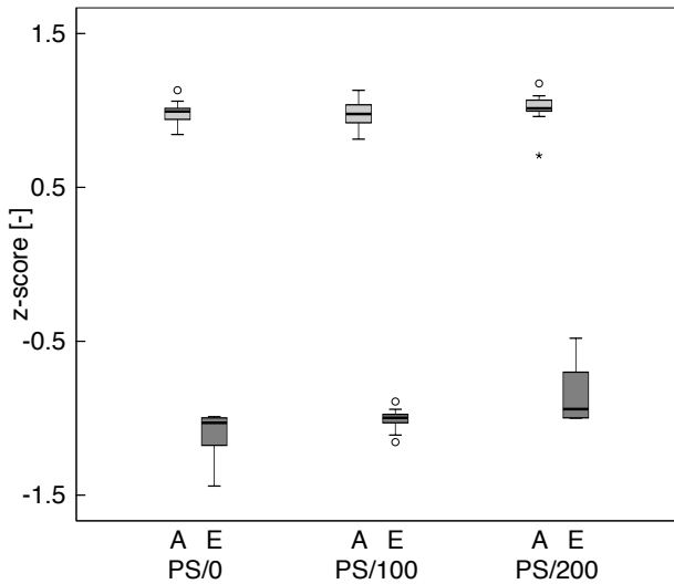
Fig. 6. Disturbed descents.
