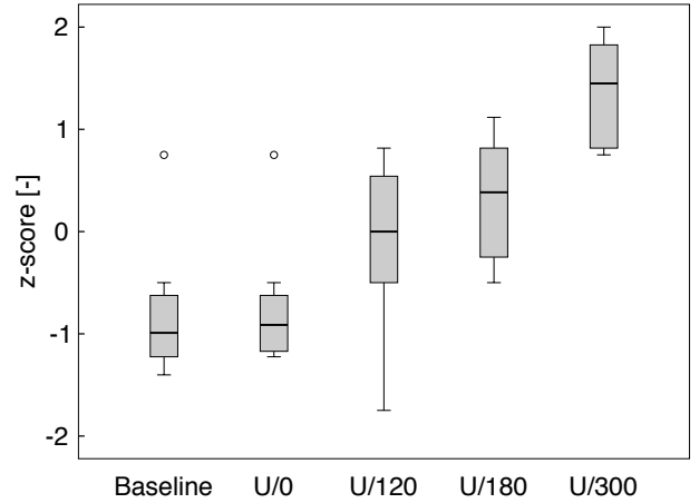
Fig. 11. Disturbed descents.
