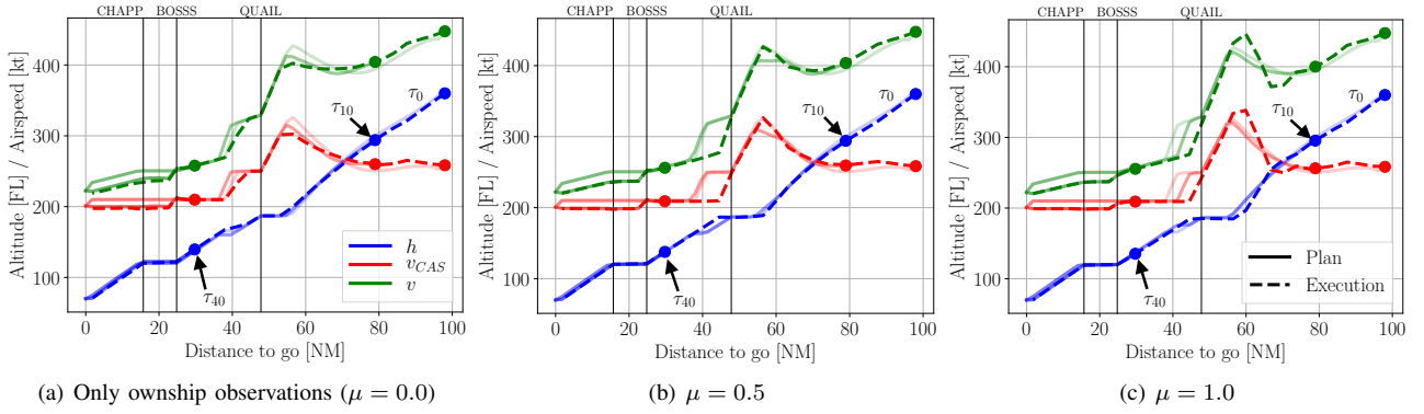
Figure 1: Planned and executed trajectories by \mu (case study 09)
