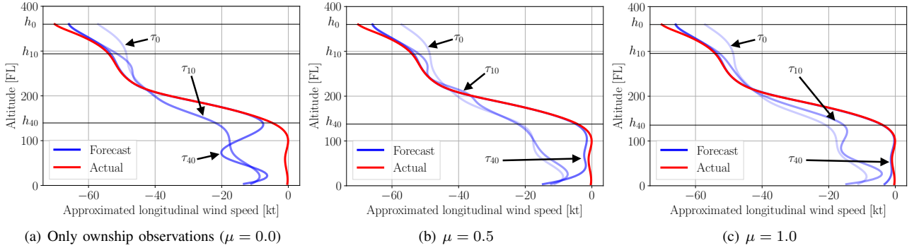
Figure 2: RAP wind forecast and analysis by \mu (case study 09)
