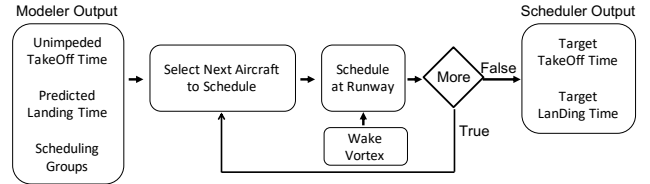
Fig. 1. High level design of the IADS scheduler.
