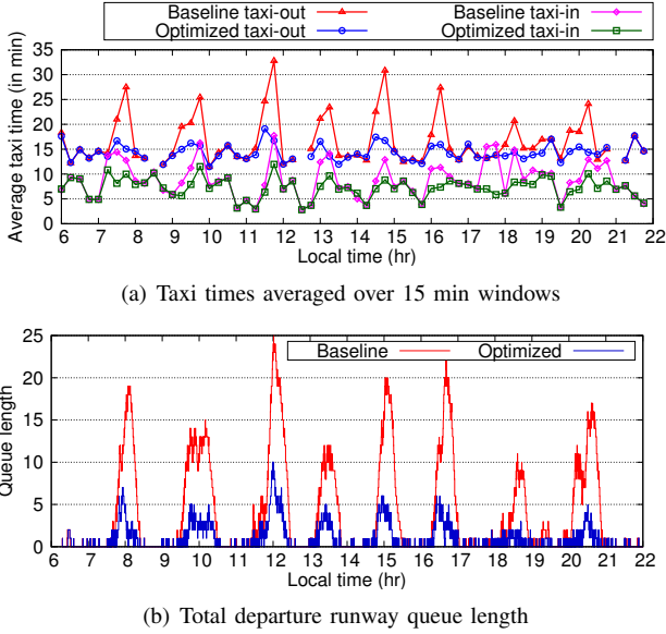
Fig. 5: Comparison of queue length and taxi-time with trajectory-based departure metering for a typical day at CLT (May 7th, 2015).
