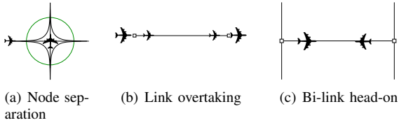
Fig. 4: Taxi separation based on node-link network.
