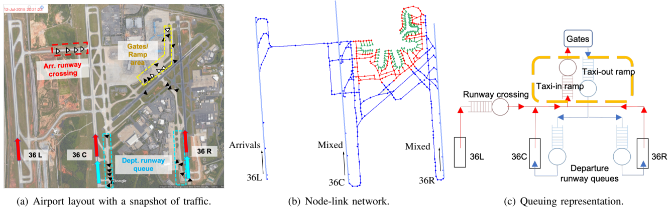
Fig. 2: CLT in North-flow runway configuration [24].
