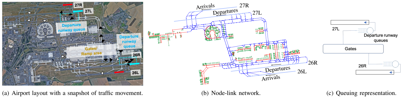
Fig. 1: CDG in West-flow runway configuration.
