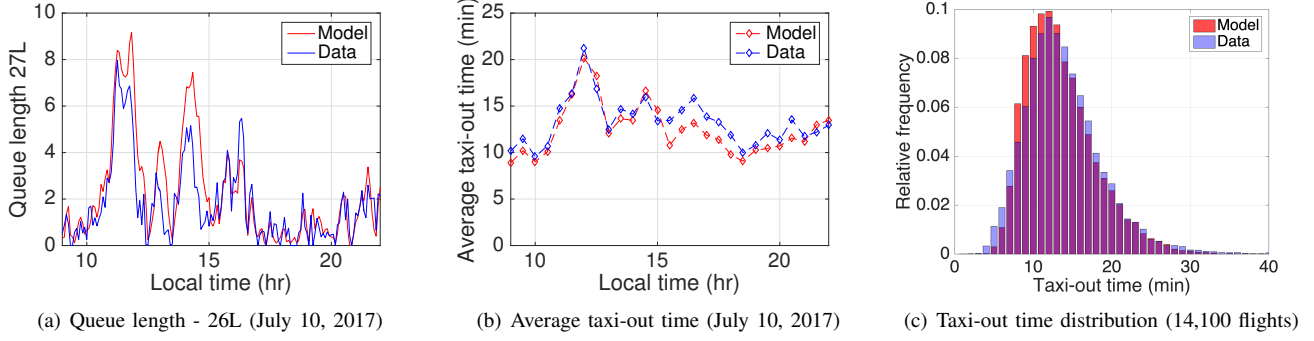
Fig. 6: Comparison between model predictions and data for CDG.
