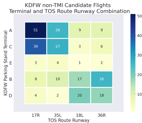
Fig. 14. KDFW non-TMI Candidate flights: combination of parking stand terminal (vertical) and TOS route runway (horizontal).
