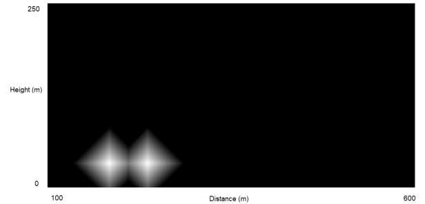
Figure 8. Blending Mask
