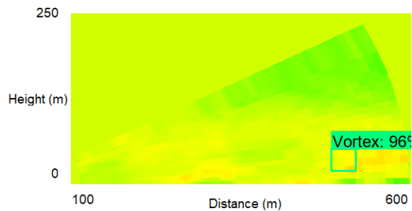
Figure 14. False Detection
