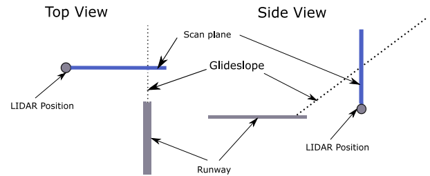
Figure 1. Scanning Geometry Overview
