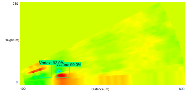
Figure 12. Two Vortices Detected on a Scan
