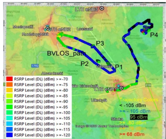
Figure 4. RSRP according to simulations at a height of 100m on the LTE 800 MHz network.
