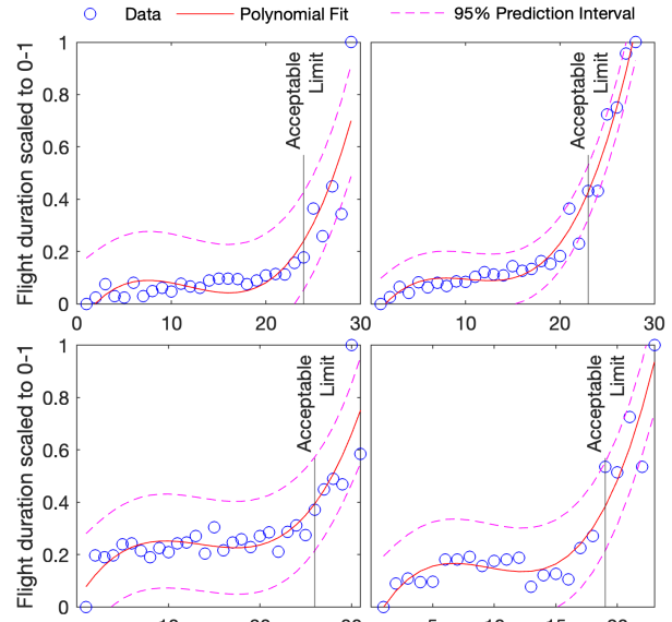
Figure 6: Flight transition duration (y-axis) versus the flow demand (x-axis) on four NFIs. The black vertical lines show the acceptable flow limit of the NFIs.
