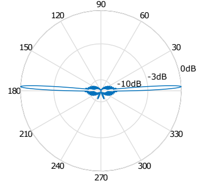
Figure 4. Tx antenna vertical radiation pattern at 1087.5 MHz.
