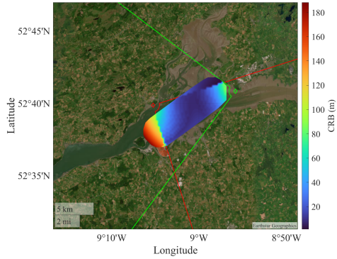
Figure 10. CRB with 2 radars
