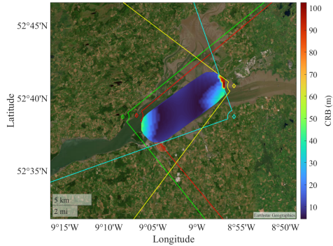
Figure 11. CRB with 4 radars
