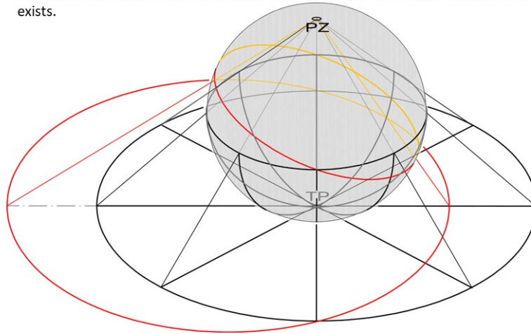
Figure 16 Principle of stereographic projection 3
