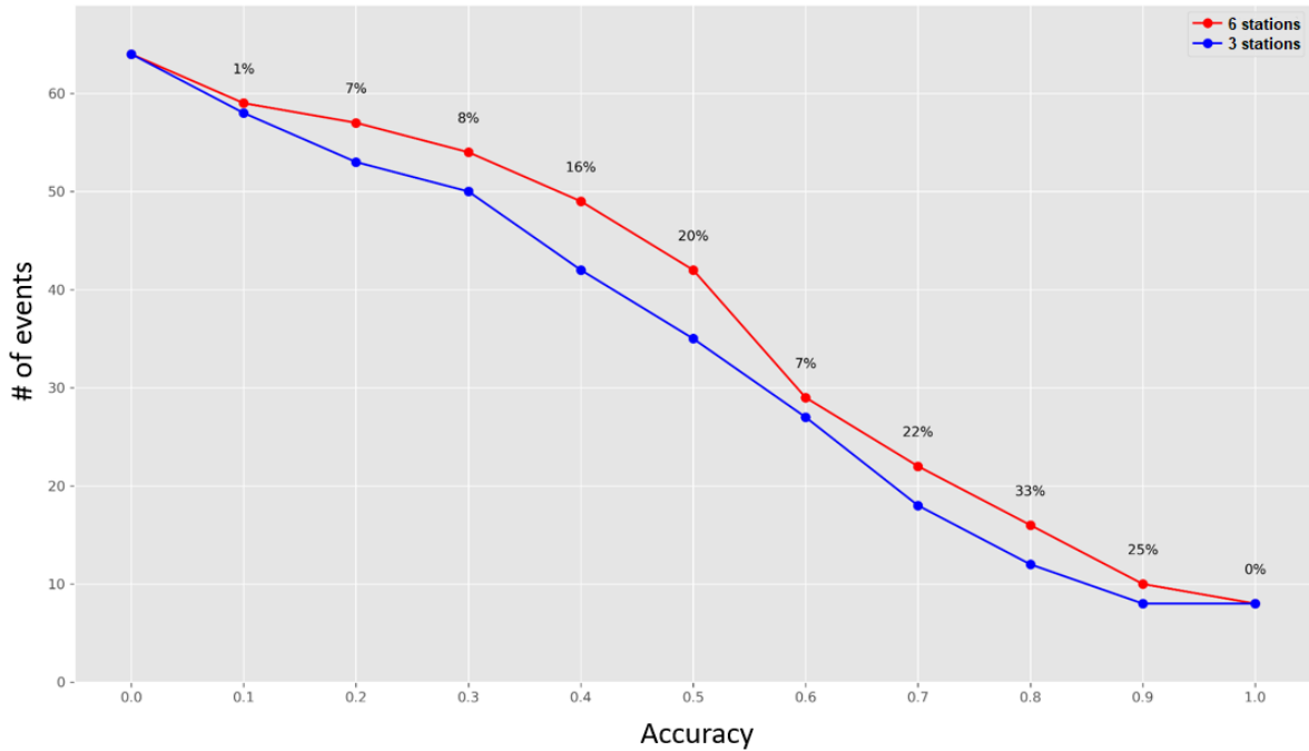
Figure 7. Survival of the nowcasting of extreme events by using as NN input the ZTD from 3 or 6 GNSS stations.
